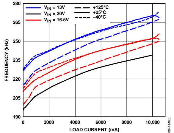
Figure 26. Frequency vs. Load Current, 300 kHz, V OUT = 0.8 V
