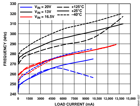
Figure 27. Frequency vs. Load Current, 300 kHz, V OUT = 1.8 V
