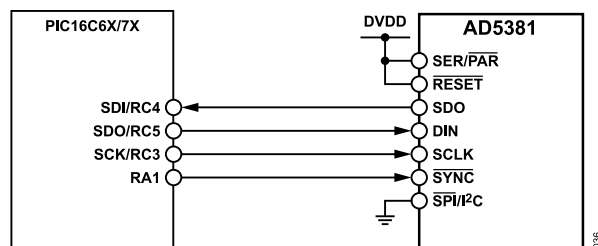
Figure 36. AD5381-to-PIC16C6x/7x Interface
