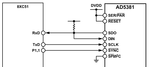
Figure 37. AD5381-to-8051 Interface
