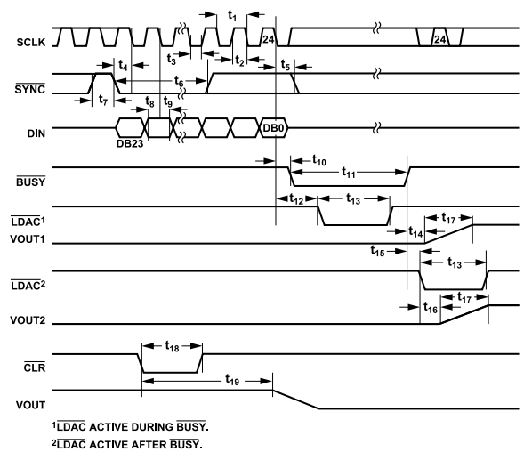
Figure 3. Serial Interface Timing Diagram (Standalone Mode)
