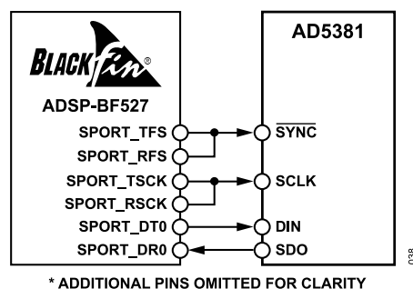
Figure 38. AD5381-to-ADSP-BF527 Interface
