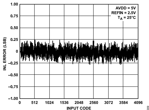
Figure 9. Typical AD5381-5 INL Plot
