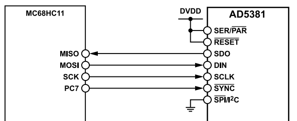
Figure 34. AD5381-to-MC68HC11 Interface
