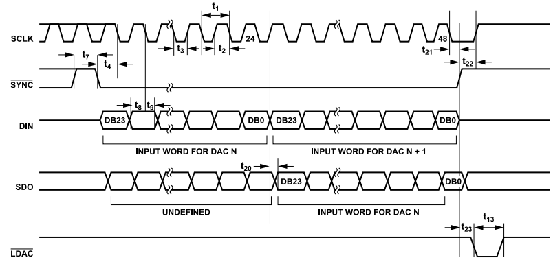
Figure 5. Serial Interface Timing Diagram (Daisy-Chain Mode)
