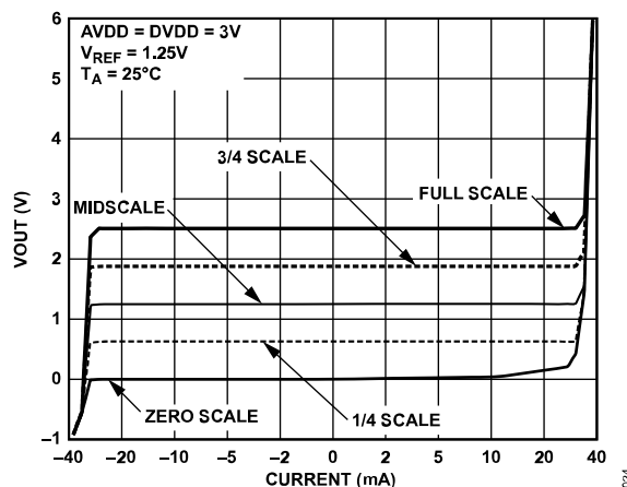
Figure 24. AD5381-3 Output Amplifier Source and Sink Capability
