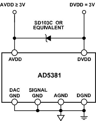
Figure 40. DVDD First Followed by AVDD
