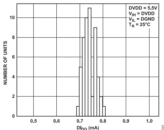
Figure 16. DI_{DD} Histogram
