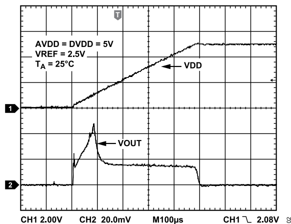
Figure 18. Power-Up Transient
