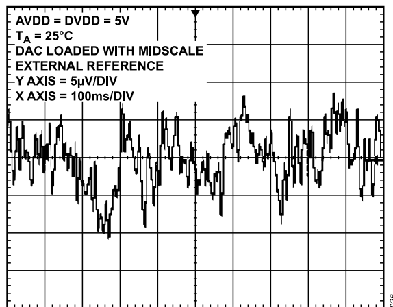
Figure 26. 0.1 Hz to 10 Hz Noise Plot
