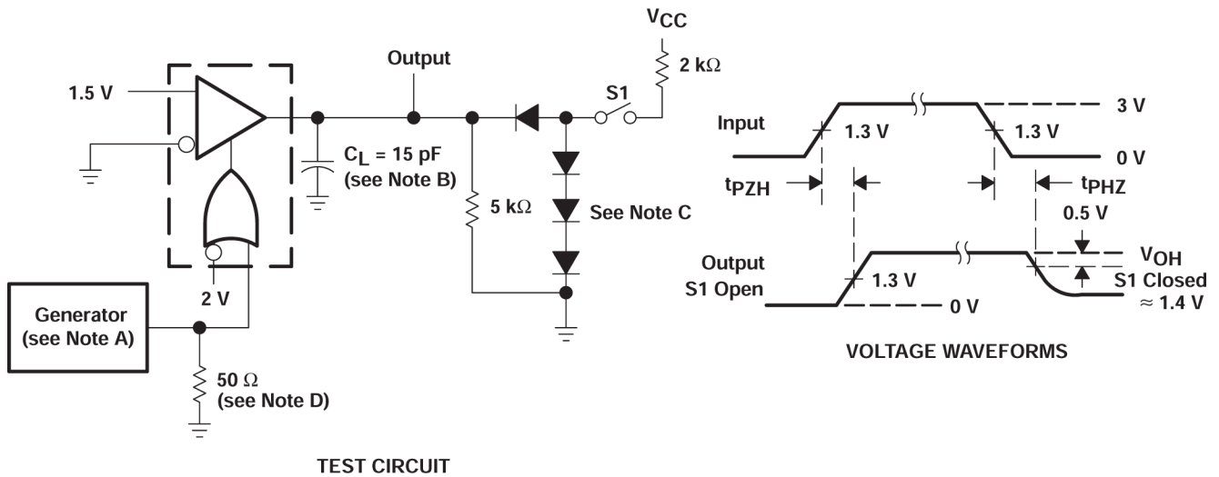
TEST CIRCUIT
