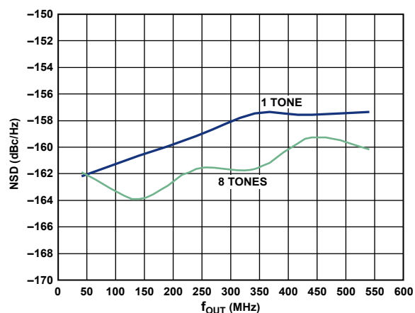
Figure 63. AD9735 NSD vs. f_{OUT} , 1.2 GSPS
