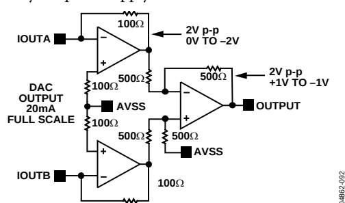
Figure 94. Op Amp I to V Conversion Output Circuit
