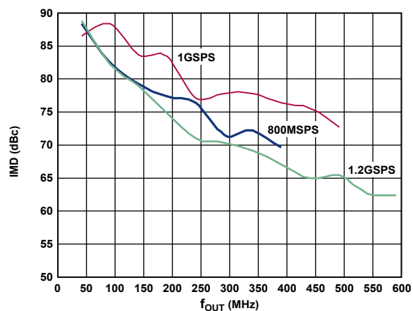
Figure 62. AD9734 IMD vs. f_{OUT} over f_{DAG} 1.2 GSPS
