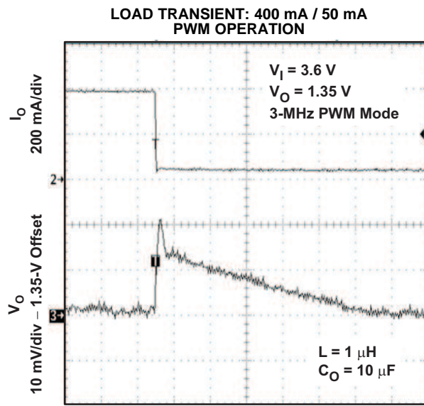
t - Time = 5 \mu\text{s}/\text{div}
