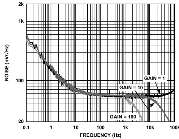
Figure 43. Voltage Noise Spectral Density vs. Frequency, RTI
