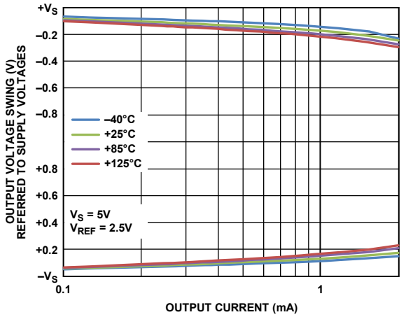
Figure 40. Output Voltage Swing vs. Output Current, V_S = 5\text{ V}
