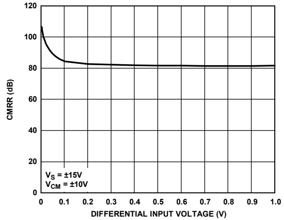
Figure 30. CMRR vs. Differential Input Voltage
