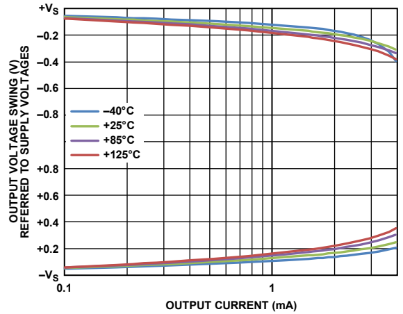
Figure 42. Output Voltage Swing vs. Output Current, V_S = \pm 15\text{ V}
