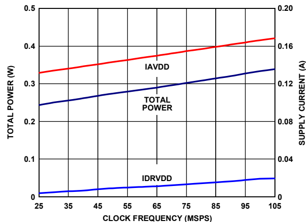
Figure 82. AD9265-105 Power and Current vs. Sample Rate
