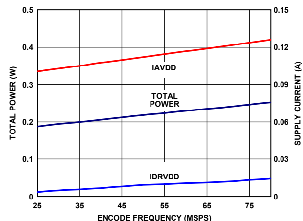
Figure 83. AD9265-80 Power and Current vs. Sample Rate
