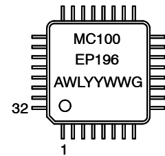
LQFP-32, 7 x 7 FA SUFFIX CASE 561AB-01
