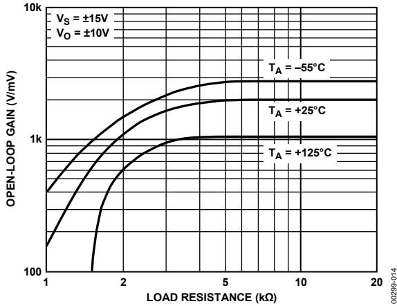
Figure 14. Open-Loop Gain vs. Load Resistance
