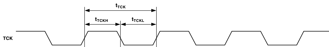
Figure 12. Reference Clocks—Test Clock (TCK) Cycle Time
