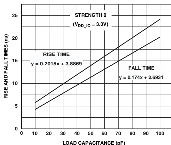
Figure 32. Typical Output Rise and Fall Time (10%-90%, V_{DD\_IO} = 3.3 V) vs. Load Capacitance at Strength 0
