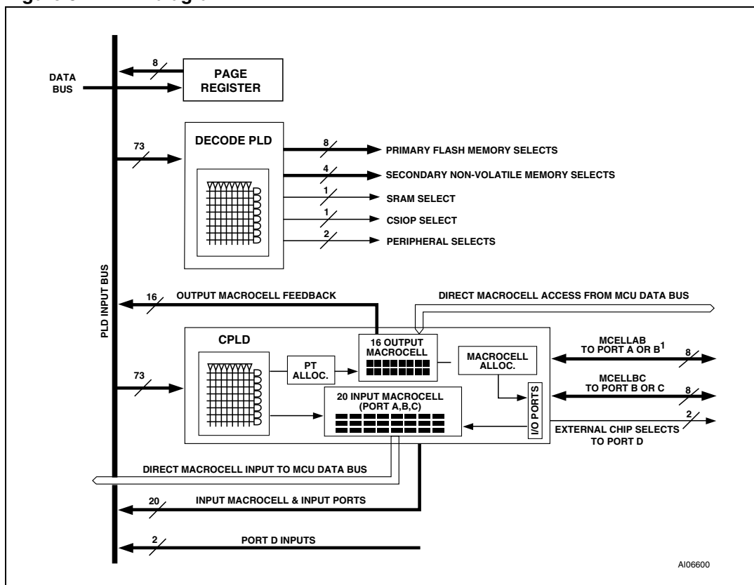
Figure 57. PLD diagram
