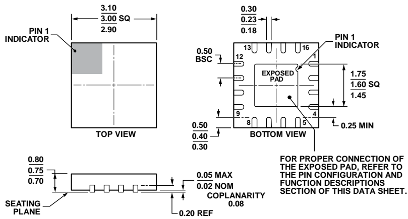
COMPLIANT TO JEDEC STANDARDS MO-220-WEED-6. Figure 53. 16-Lead Lead Frame Chip Scale Package [LFCSP_WQ] 3 mm x 3 mm Body, Very Very Thin Quad (CP-16-22) Dimensions shown in millimeters
