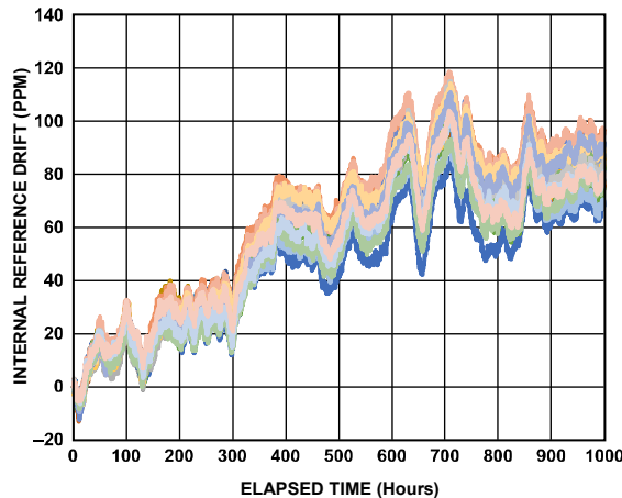
Figure 48. Reference Drift Through to 1000 Hours
