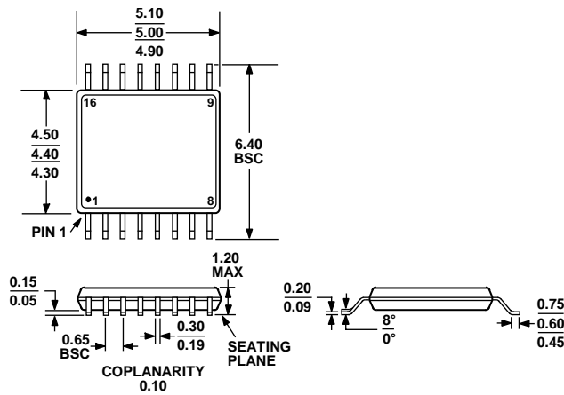
COMPLIANT TO JEDEC STANDARDS MO-153-AB Figure 54. 16-Lead Thin Shrink Small Outline Package [TSSOP] (RU-16) Dimensions shown in millimeters
