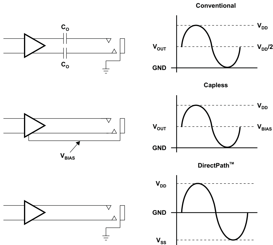
Figure 34. Amplifier Applications
