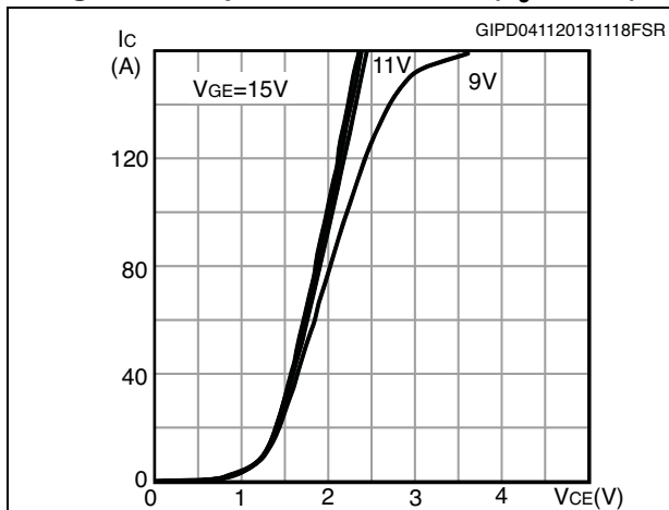
Figure 4. Output characteristics ( T_J = 25\text{ °C} )
