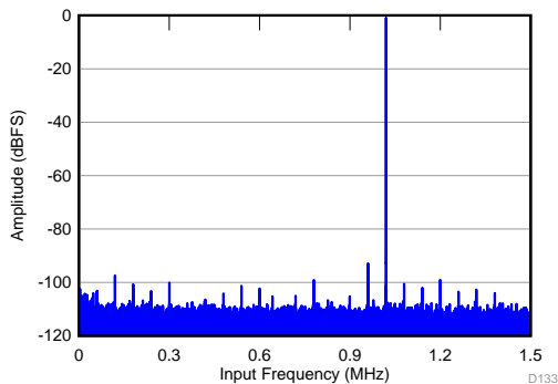
Figure 136. FFT for 3-MSPS Sampling Speed
