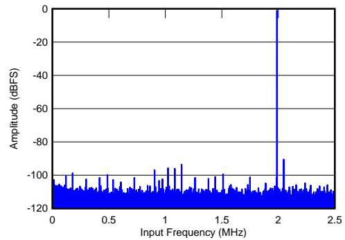
Figure 137. FFT for 5-MSPS Sampling Speed
