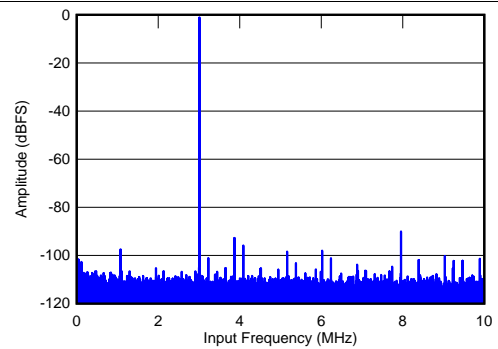
Figure 139. FFT for 10-MSPS Sampling Speed
