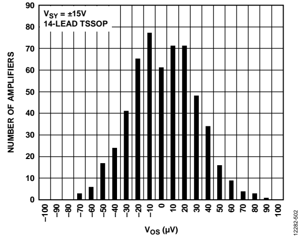
Figure 18. Input Offset Voltage ( V_{OS} ) Distribution, V_{SY} = \pm 15V , 14-Lead TSSOP
