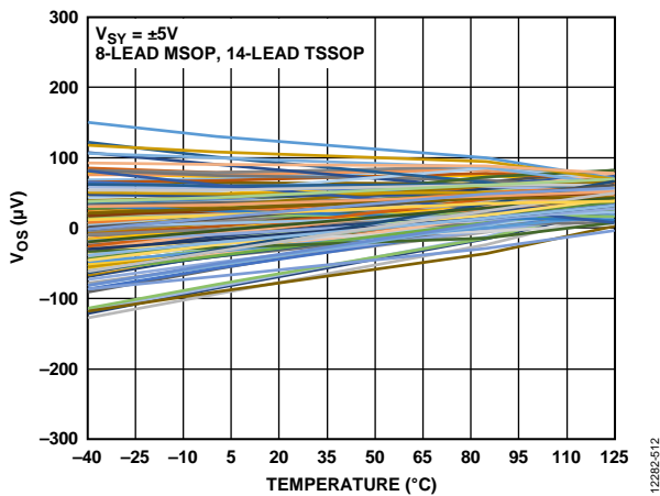
Figure 17. Input Offset Voltage ( V_{OS} ) vs. Temperature, V_{SY} = \pm 5V , 8-Lead MSOP and 14-Lead TSSOP
