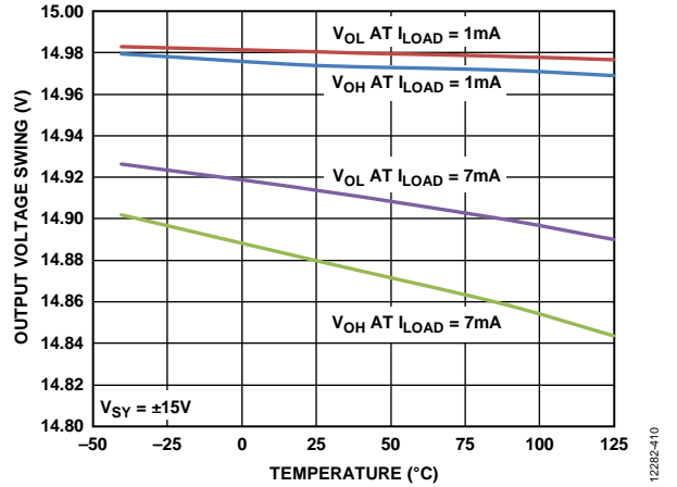
Figure 30. Output Voltage Swing vs. Temperature, V_{SY} = \pm 15V
