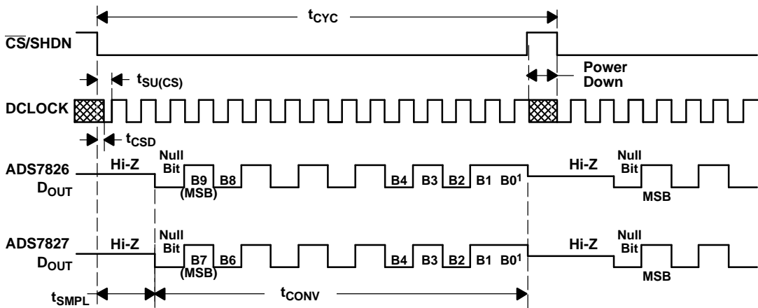
Figure 37. ADS7826 and ADS7827 Timing
