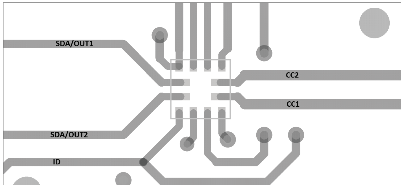
Figure 16. TUSB320 Layout
