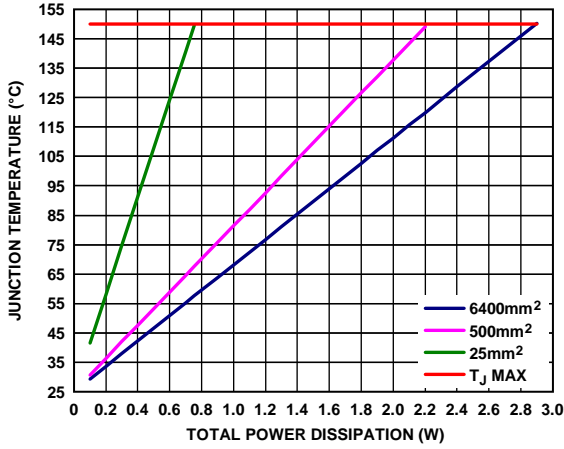
Figure 64. LFCSP, TA = 25°C
