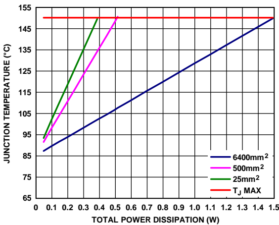
Figure 66. LFCSP, TA = 85°C
