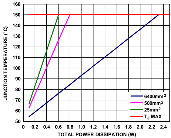
Figure 65. LFCSP, TA = 50°C
