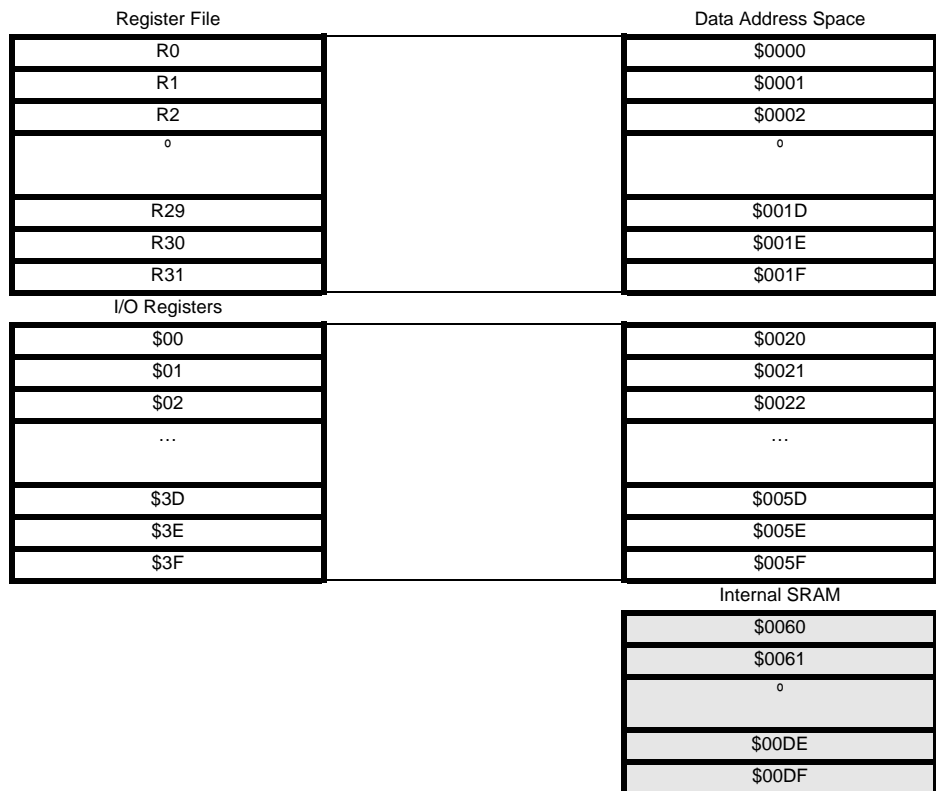
Figure 9. SRAM Organization
