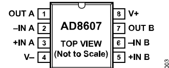
Figure 3. 8-Lead SOIC (R Suffix)
