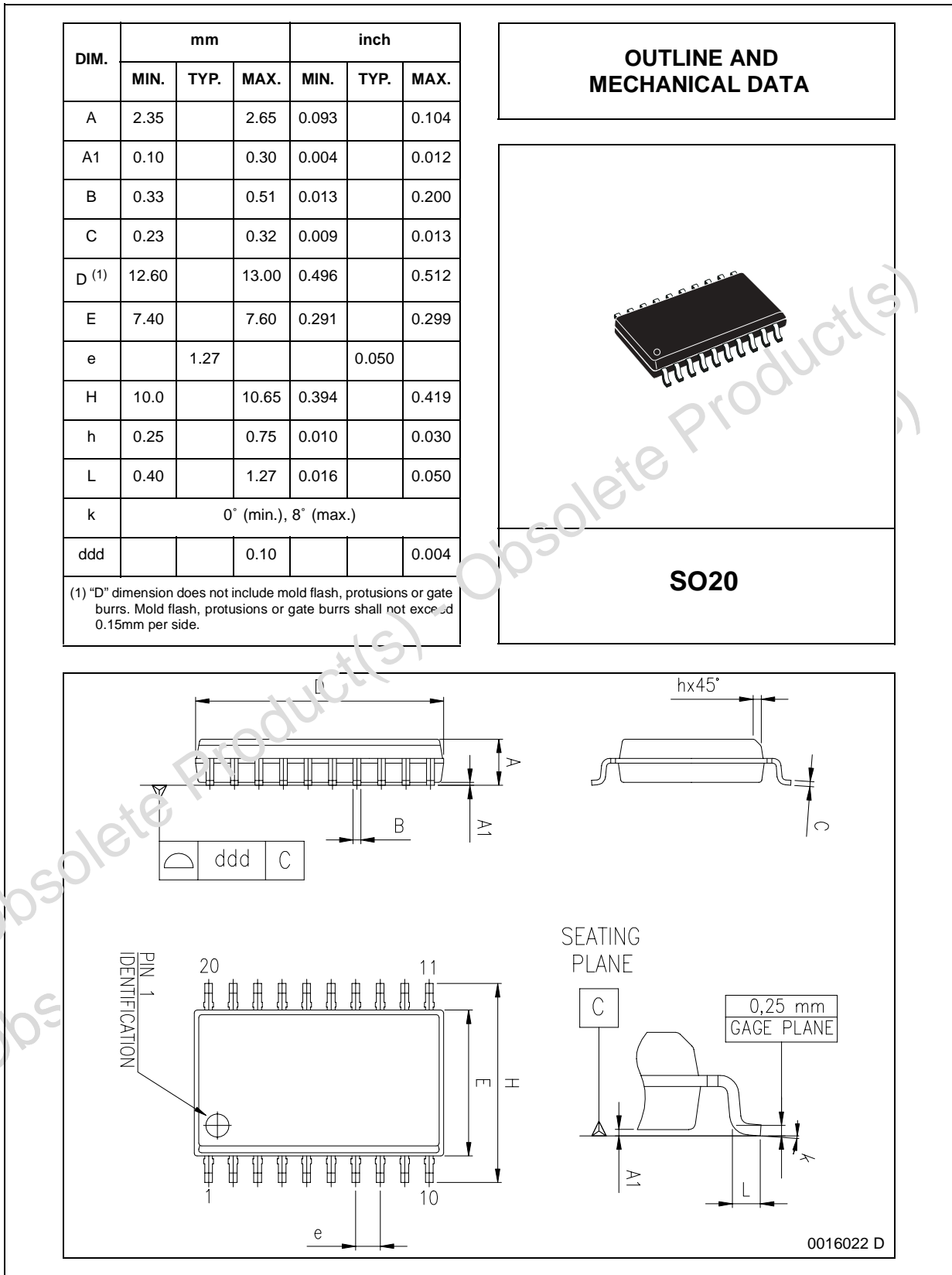
Figure 15. SO20 Mechanical Data & Package Dimensions
