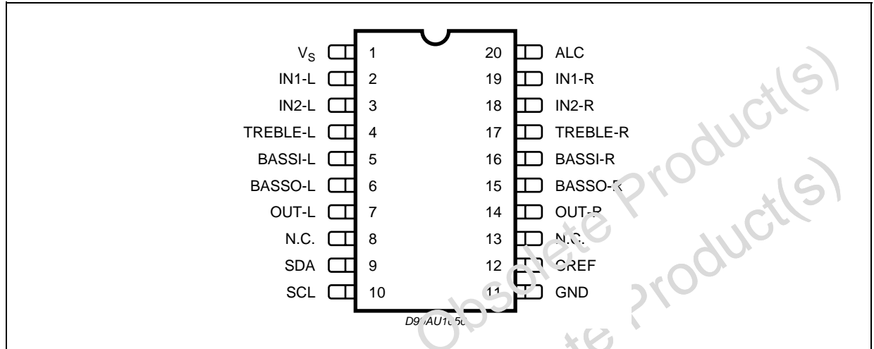
Figure 3. Pin Connection
