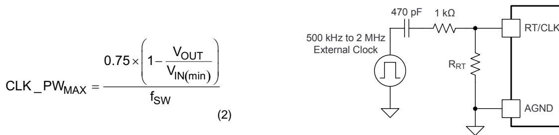
Figure 28. CLK/RT Configuration
