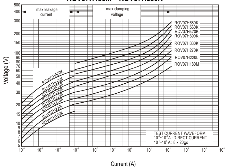
ROV07H180M – ROV07H680K
