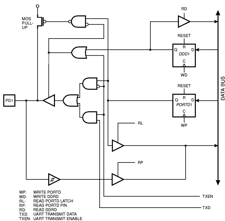
Figure 54. Port D Schematic Diagram (Pin PD1)
