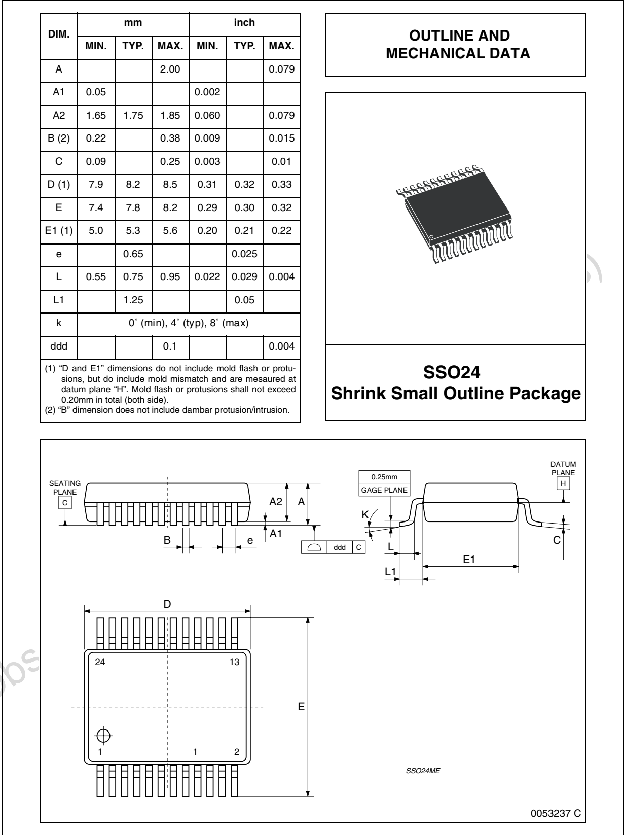
Figure 12. SSO24 Mechanical Data & Package Dimensions
