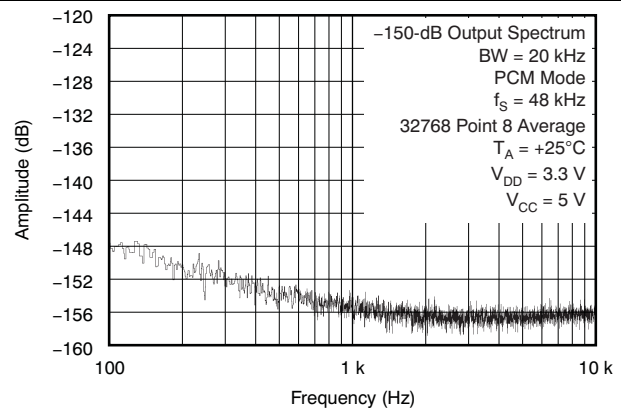
Figure 23. Amplitude vs Frequency (Measurement Circuit: Figure 53 )
