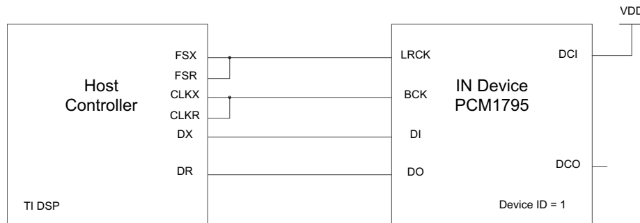
Figure 68. TDMCA Diagram
