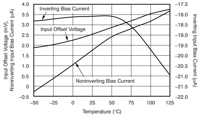
TYPICAL DC DRIFT OVER TEMPERATURE
