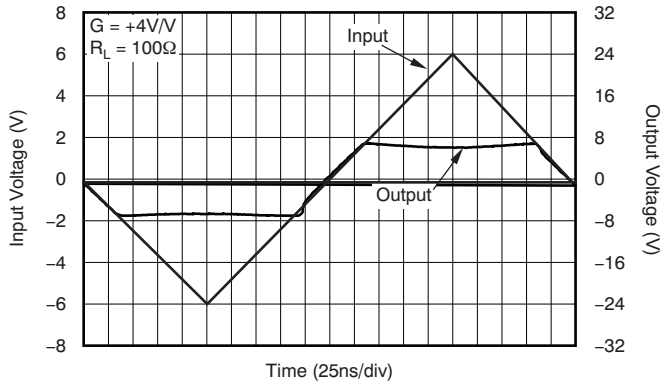
OVERDRIVE RECOVERY
