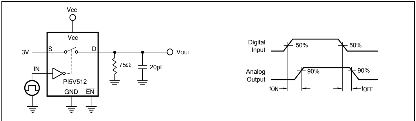
Figure 1. Switching Time
