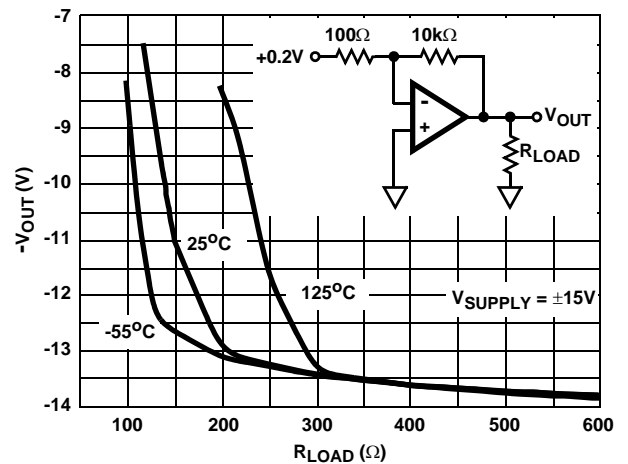
FIGURE 21. -V OUT vs R L
