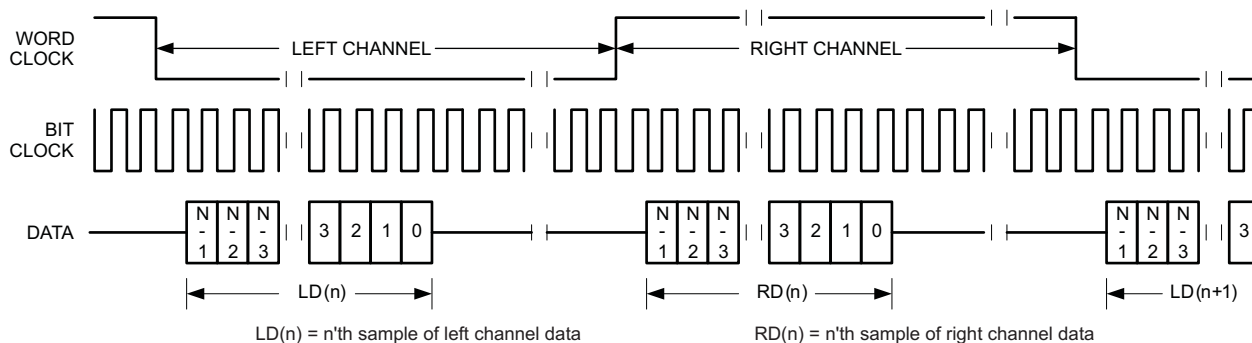
Figure 6-27. Timing Diagram for I 2 S Mode
