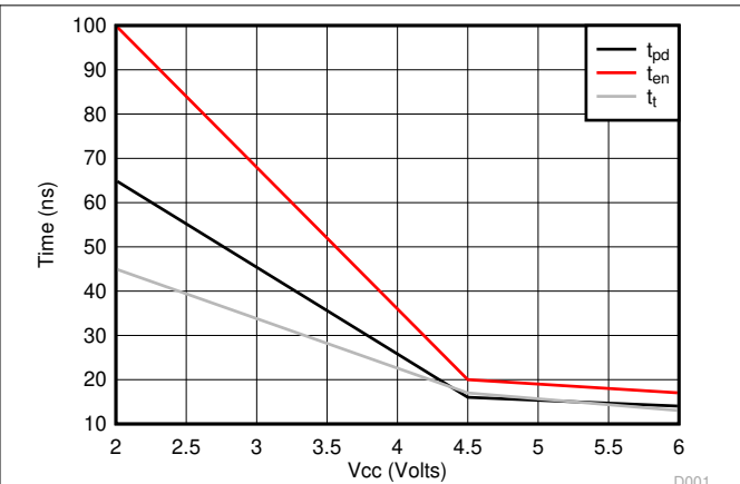
Figure 6-2. Typical Delay vs. V_{CC} for C_L = 150 pF
