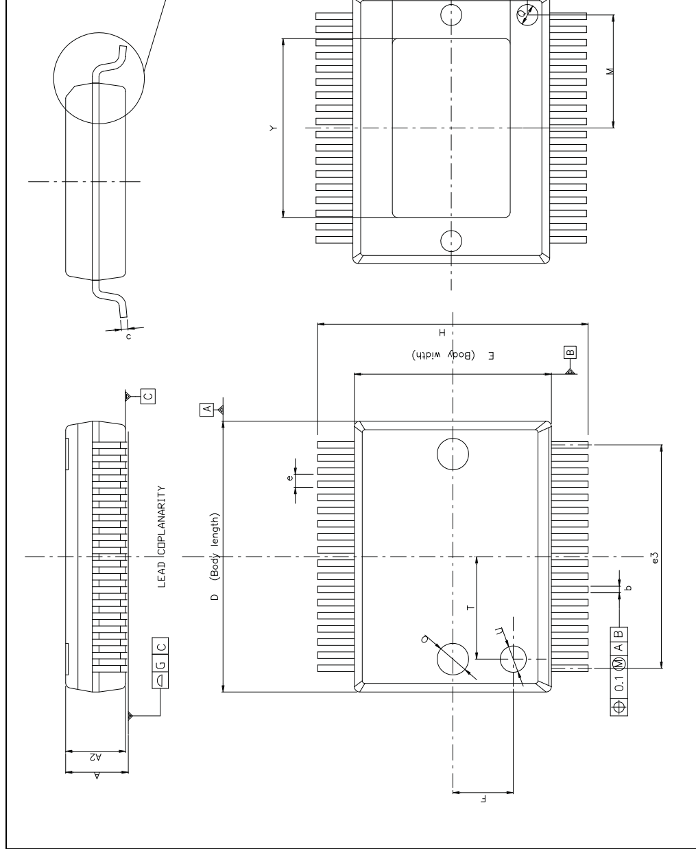
Figure 36. PowerSSO-36 EPD outline drawing
