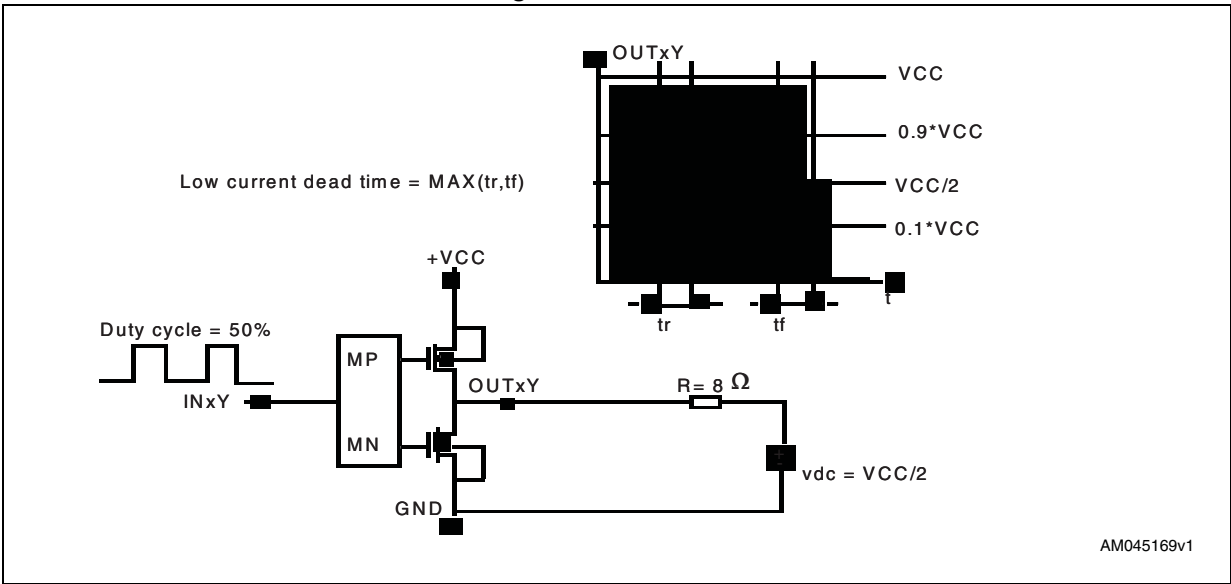
Figure 3. Test circuit
