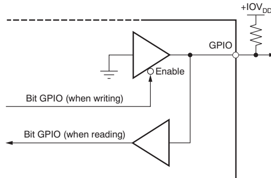
Figure 97. GPIO Pin
