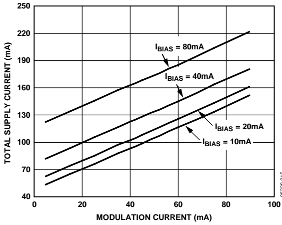
Figure 15. Total Supply Current vs. Modulation Current Total Supply Current = I_{CC} + I_{BIAS} + I_{MOD}
