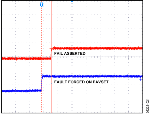
Figure 21. FAIL Assert Time, 1 μs/DIV
