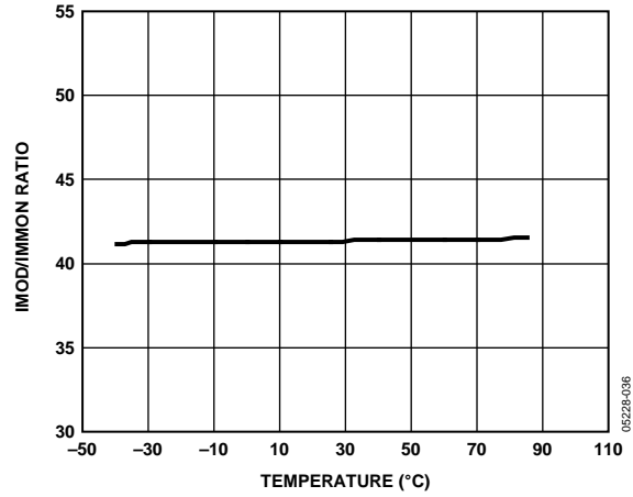
Figure 19. I_{MOD}/I_{MMON} Gain vs. Temperature, I_{MOD} = 30\text{ mA}
