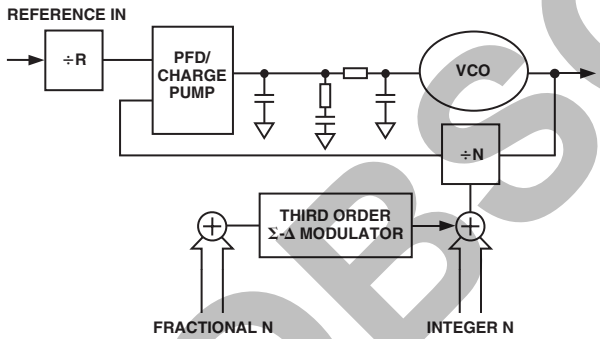
Figure 11. Fractional-N PLL
