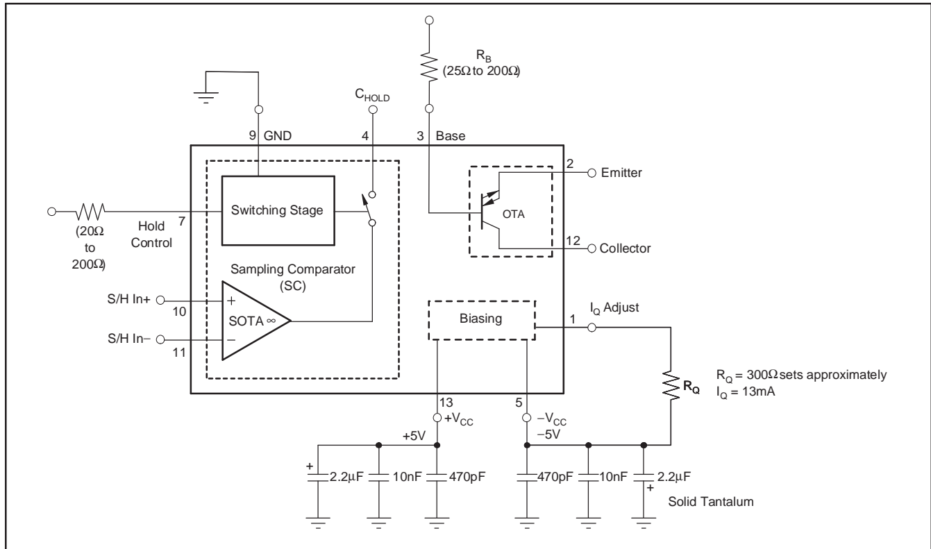
Figure 39. Basic Connections
