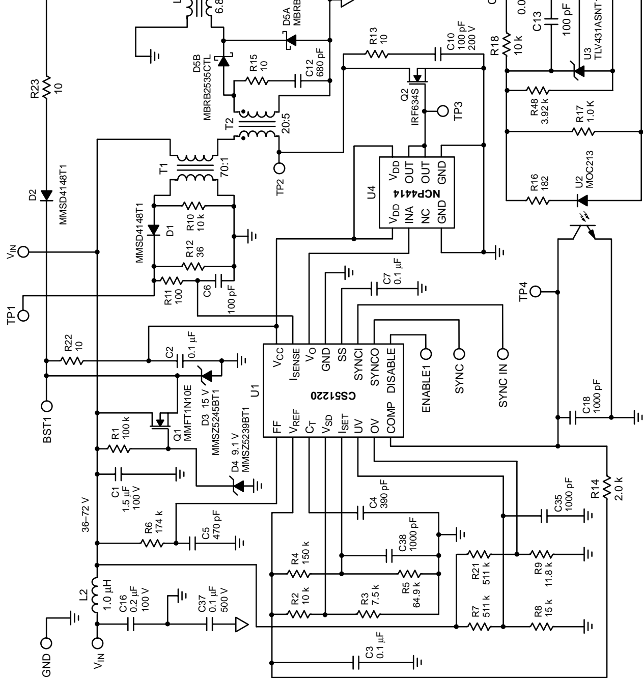
Figure 17. Additional Application Diagram, 5.0 V Output Converter Used As Sync Master for the Dual Converter
