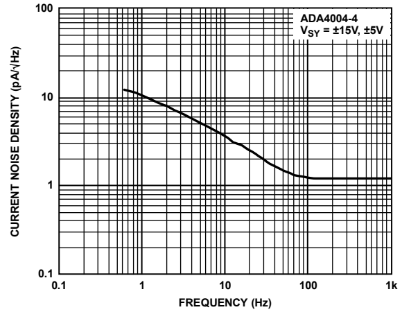
Figure 38. Current Noise Density vs. Frequency
