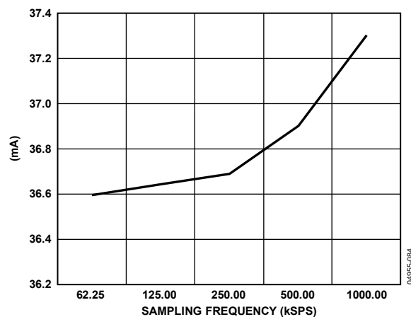
Figure 43. Current Consumption vs. Sampling Frequency
