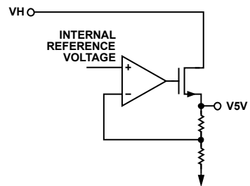
Figure 12. V5V
