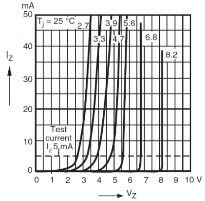
Fig. 14 - Breakdown Characteristics
