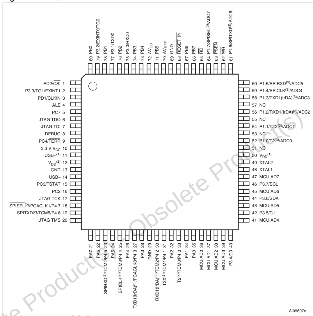
Figure 3. LQFP80 connections
