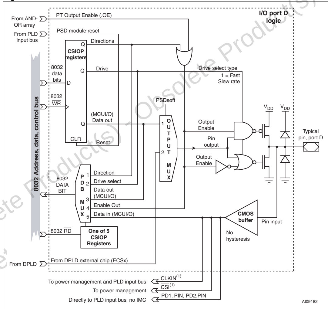
Figure 87. Port D structure
