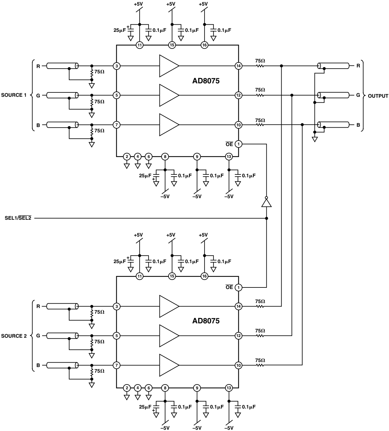
Figure 4. Mux
