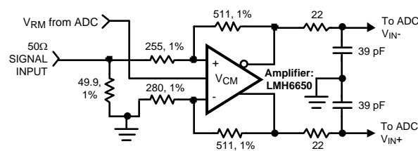
Figure 44. Optional Amplifier Drive for Circuit in Figure 43
