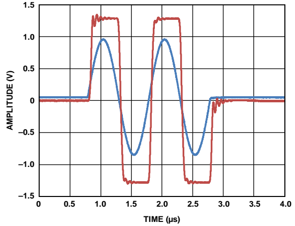
Figure 19. Overdrive Recovery
