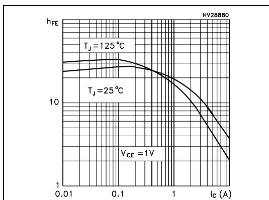
Figure 5. DC current gain @ V_{CE}=1V
