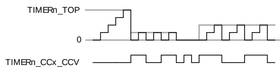
Figure 17.17. TIMER Up-count Frequency Generation
