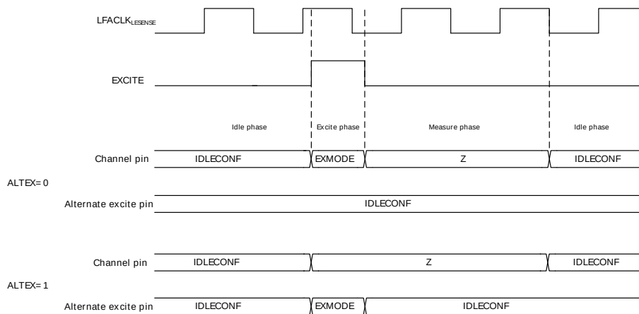
Figure 21.4. Pin sequencing
