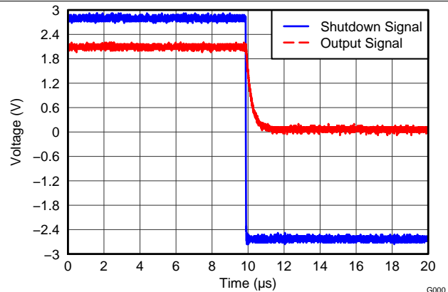
Figure 26. Turnoff Transient
