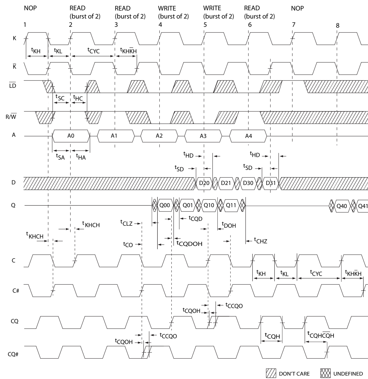
Figure 5. Read/Write/Deselect Sequence [26, 27, 28]
